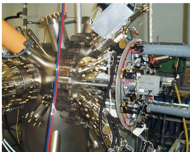
Photo 1: RF plasma-assisted molecular beam epitaxy (RF-MBE) system
