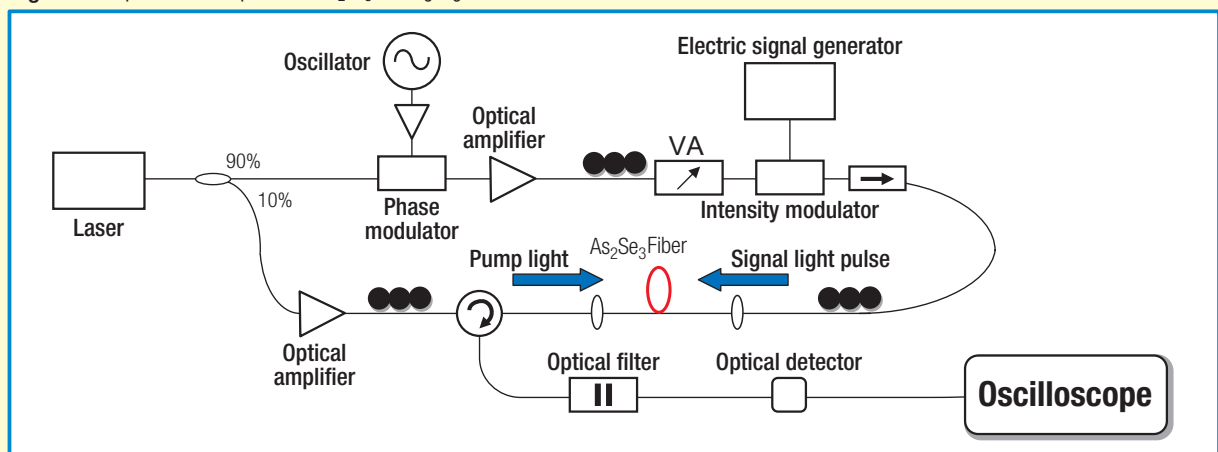
Figure 3. Experimental setup used for \text{As}_2\text{Se}_3 slow light generation
