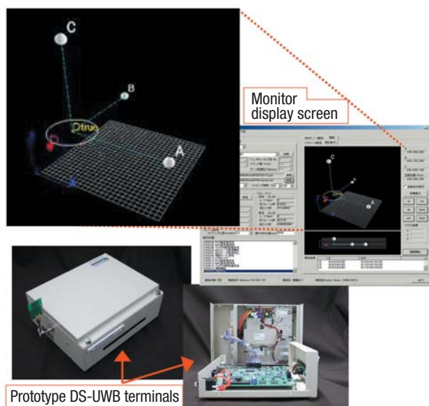
Figure 3: Prototype UWB system equipped with communication and distance measurement functions
