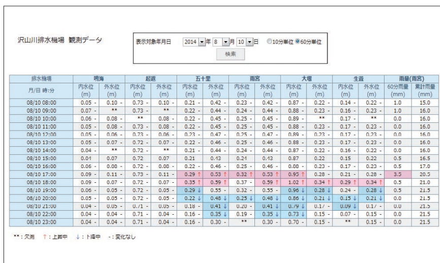
Figure 6 Measured water level data
