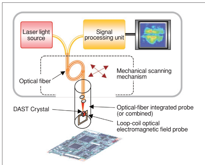
Figure 3 ● Probe-scanning Measurement System
