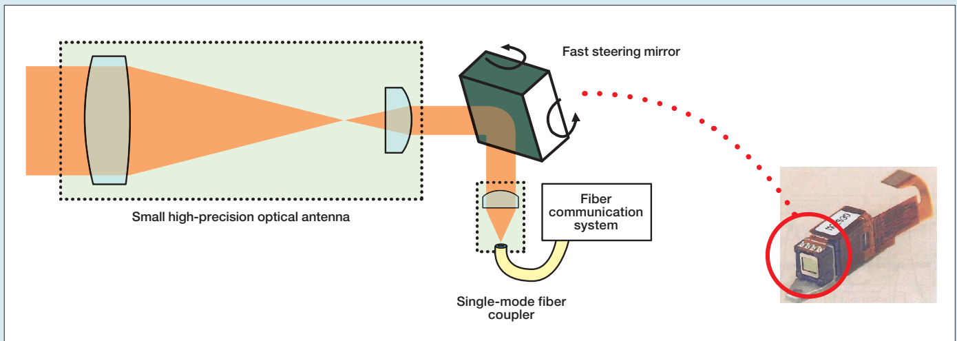
Fig. 3 ● Operating principle of the terminal Free-space laser beam will be converted to a small collimated beam and then stabilized in its direction by the fast steering mirror so that the beam focus exactly matches the center of the single mode fiber aperture.
