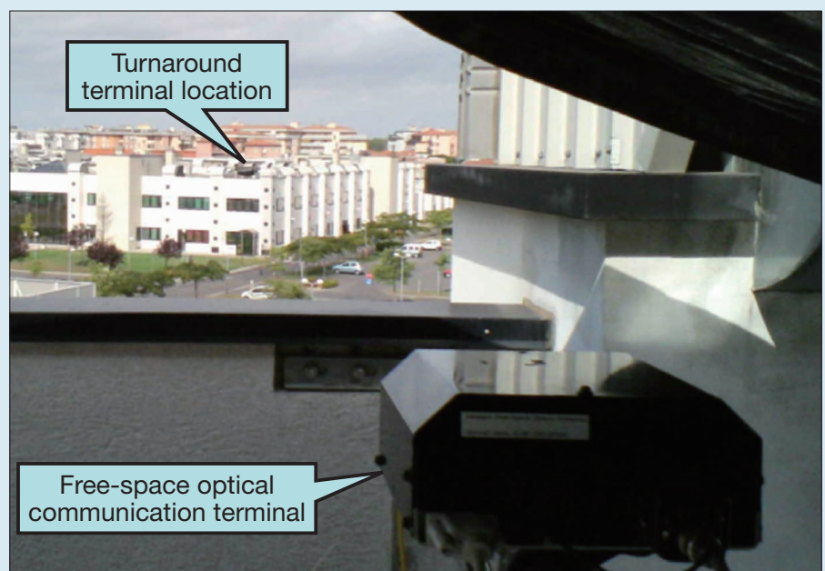
Fig. 5 ● The exterior appearance of free space optical communication system installed on the roof of Center of Excellence for Information and Communication Engineering (CEIIC), Santana University (left) and the turnaround terminal location viewed from the free space optical communication terminal (right)
