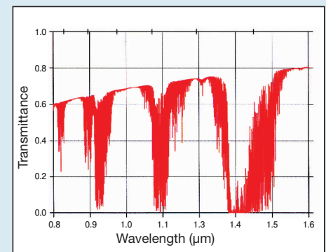
Fig. 4 ● Propagation characteristics in urban atmosphere An example of calculated absorption attenuation of laser light in 1 km horizontal propagation distance in an urban area. The longitudinal axis shows transmittance, and the abscissa axis shows wavelength. The parts of deeply declined transmittance indicate the effect of water vapor absorption. The transmittance of 0.78 \mu\text{m} or 0.85 \mu\text{m} wavelength used by conventional optical wireless communication systems is about 60%. The transmittance of 1.3 \mu\text{m} and 1.5 \mu\text{m} wavelength used by long-haul fiber optic communications and NICT's free space optical communication systems is about 80%.
