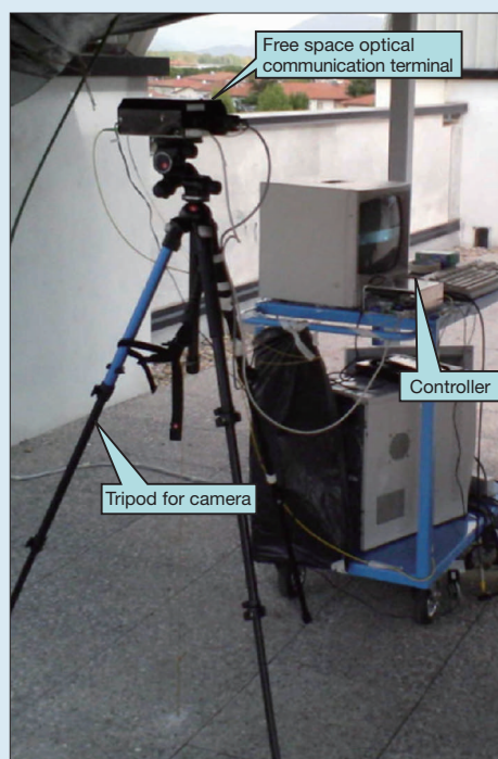
Fig. 5 ● The exterior appearance of free space optical communication system installed on the roof of Center of Excellence for Information and Communication Engineering (CEIIC), Santana University (left) and the turnaround terminal location viewed from the free space optical communication terminal (right)
