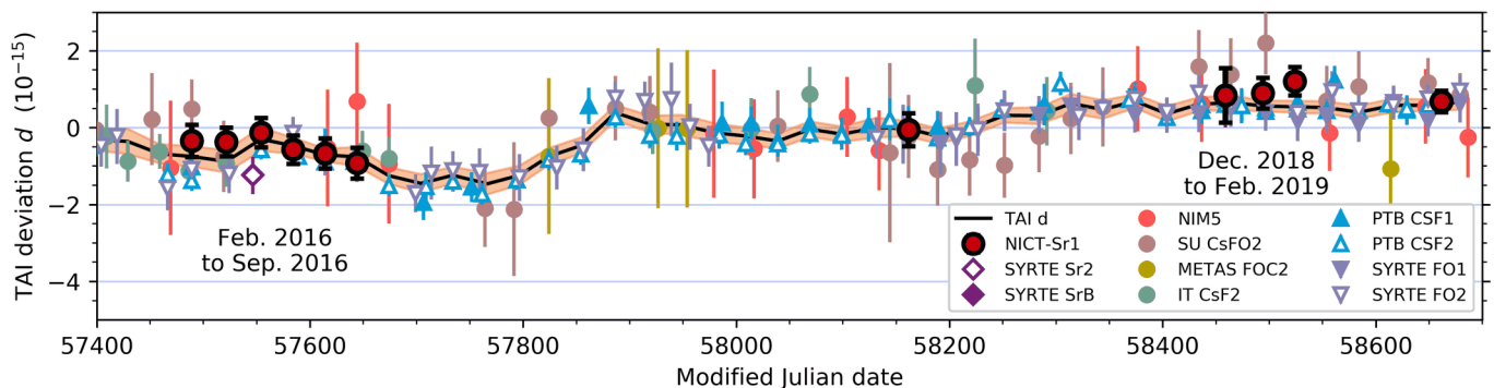
Fig. 7 Deviation d of TAI scale interval from the SI second
